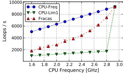
Fig. 7: Threads benchmark
