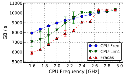
Fig. 8: STREAM benchmark
